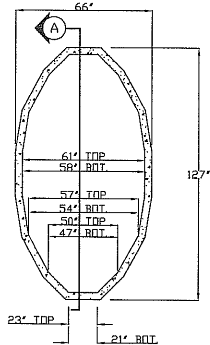
PLAN-STRUCTURE
