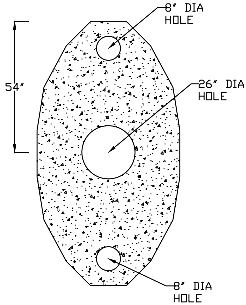
PLAN-TOP SLAB
