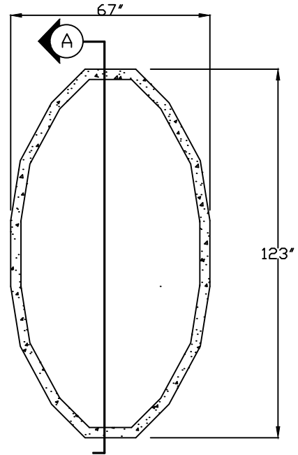
PLAN-STRUCTURE
