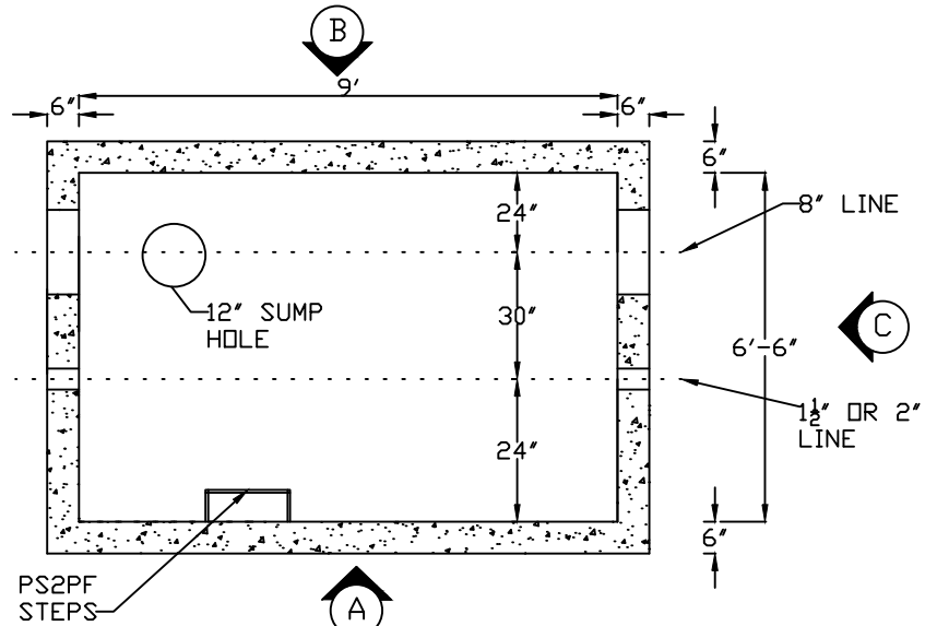
PLAN-STRUCTURE
