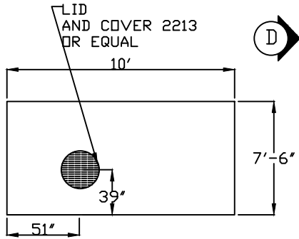
PLAN-TOP SLAB
