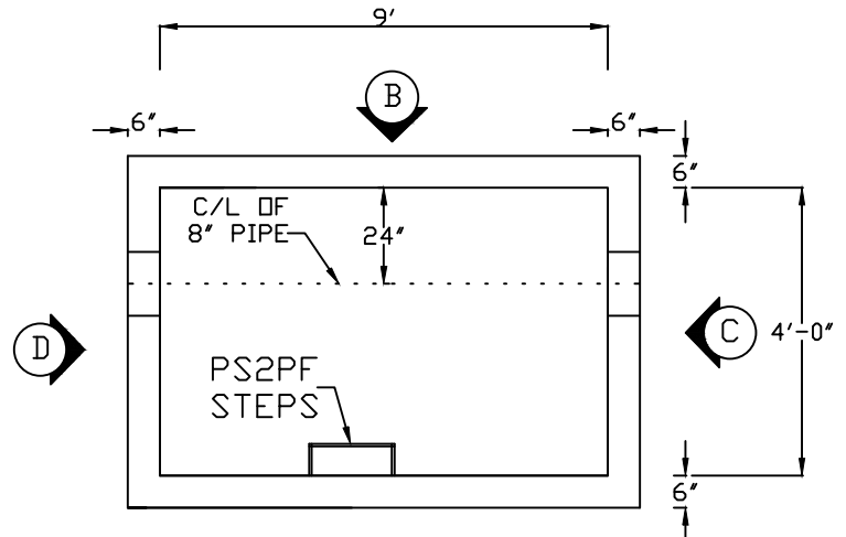
PLAN-STRUCTURE
