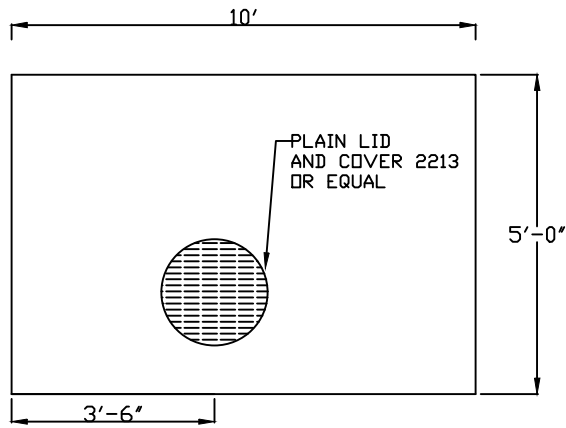
PLAN-TOP SLAB
